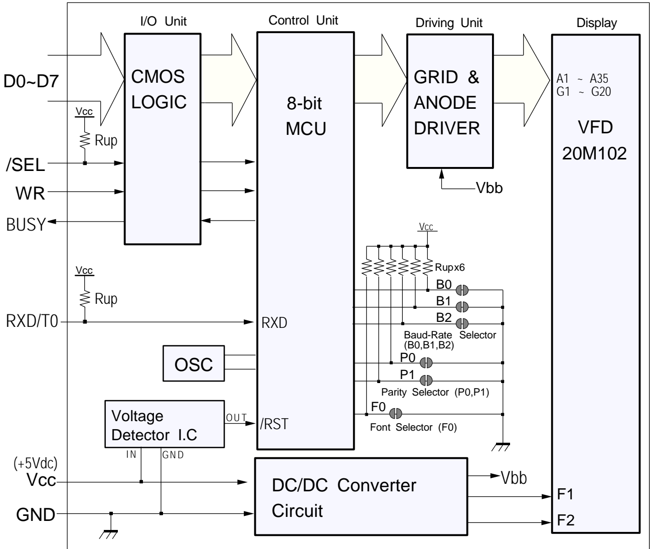
Fig-5. VFD Module System Block Diagram
