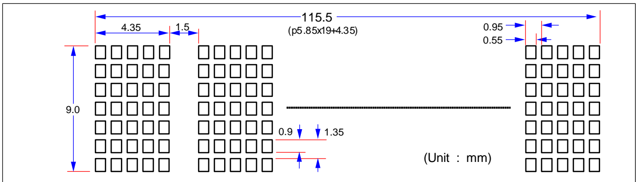
Fig-4. Pattern Details
